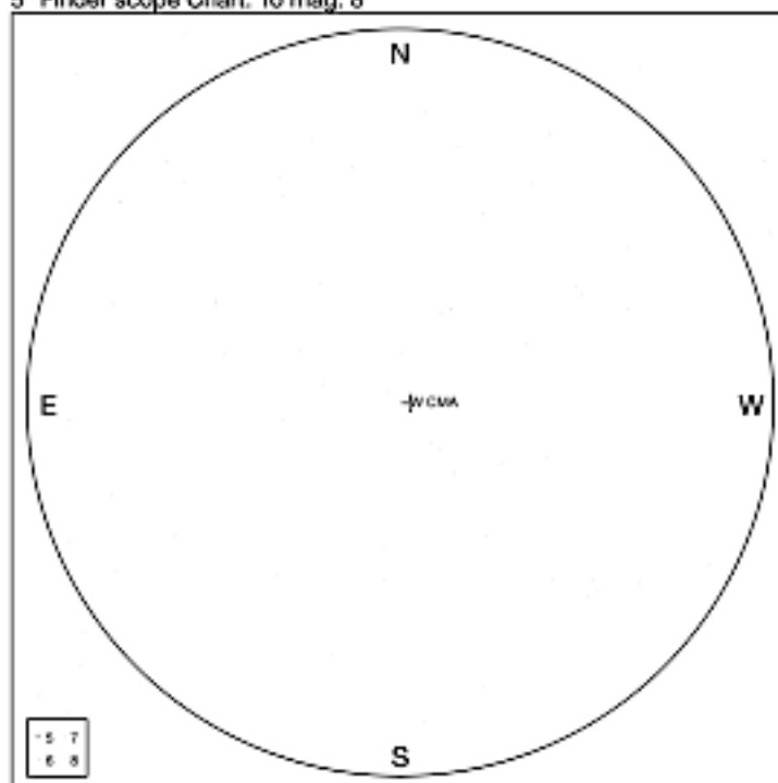
5° Finder scope Chart. To mag: 8
