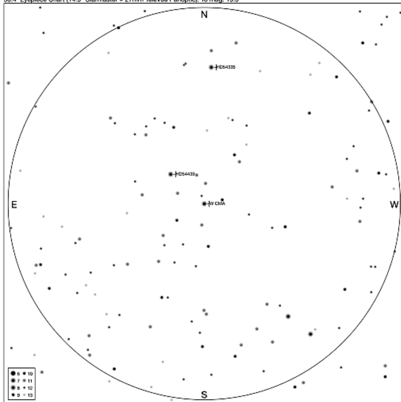
56.4' Eyepiece Chart (14.5° Starmaster + 27mm TeleVue Panoptic). To mag: 15.5
